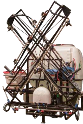
Midi-Spray Mounted 600 litre PRO spec with 6m 3-section heavy duty folding boom and retracting hose reel with hand lance
