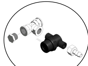
SP/SP/MS003/7/9/FILTER Filter spares kit
